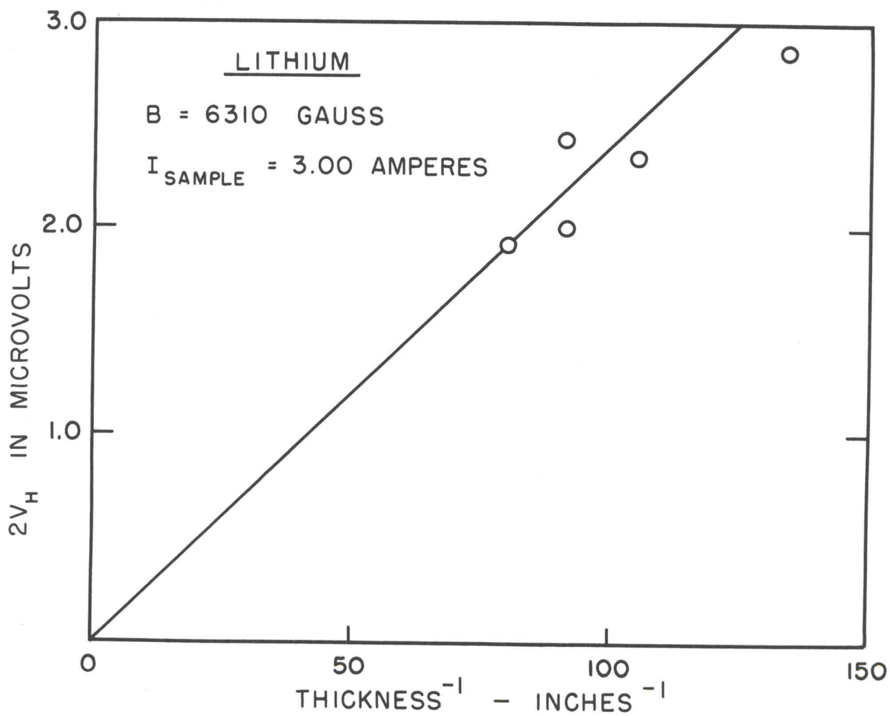
FIG. 3-16 HALL VOLTAGE \times 2 , 2V_H , VS. SAMPLE THICKNESS -1
